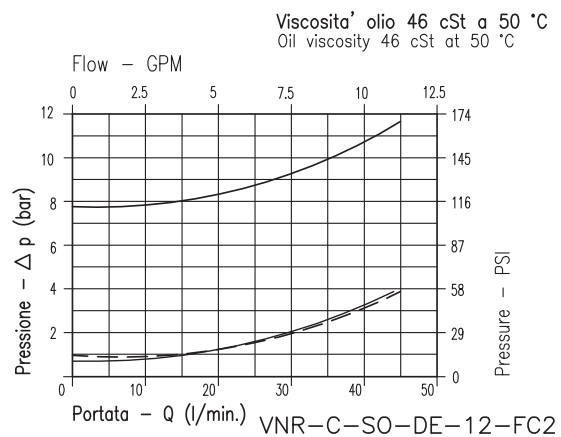
Viscosità olio 46 cSt a 50°C / Oil viscosity 46 cSt at 50°C
